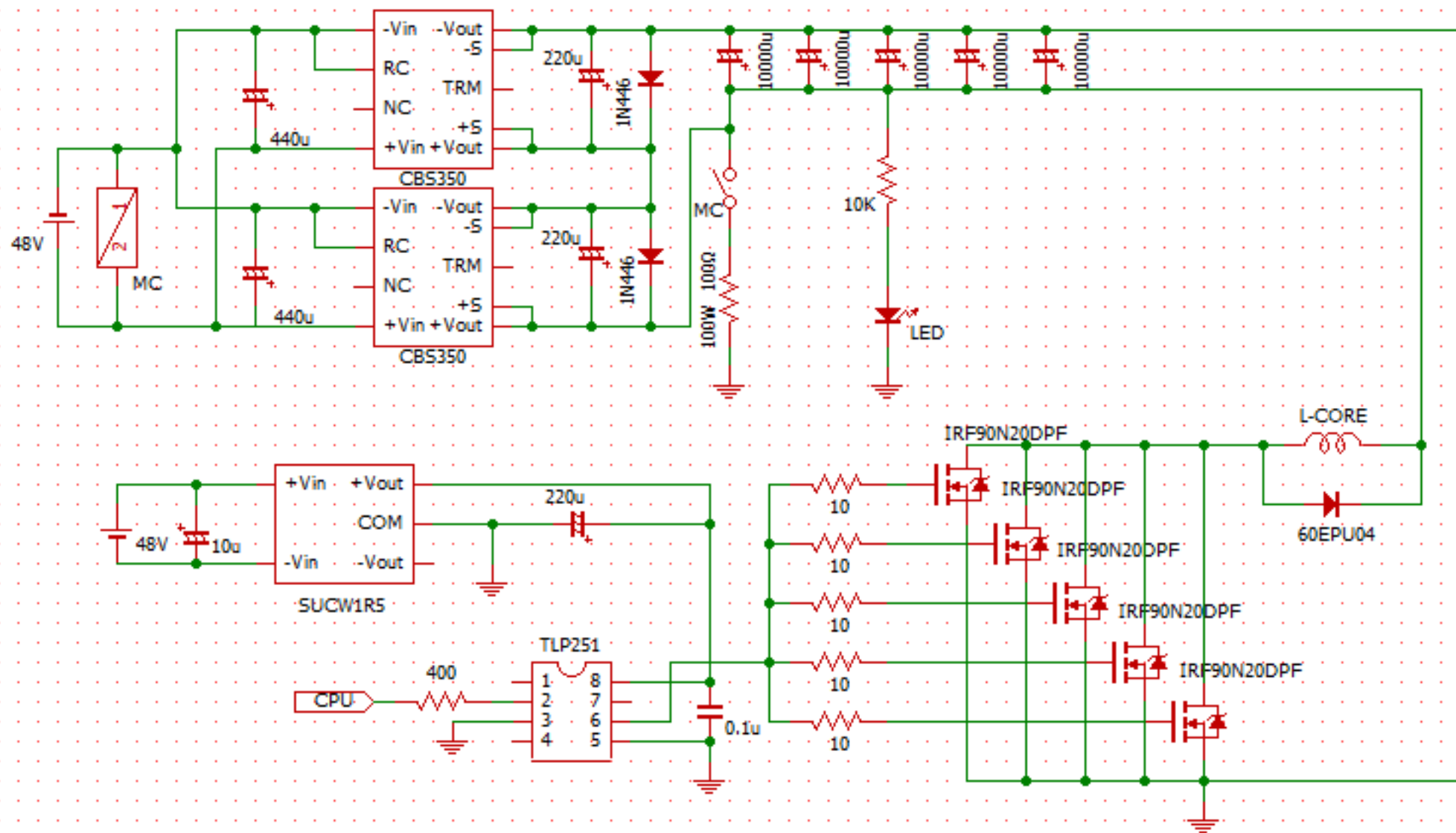
Circuit for kicking module
